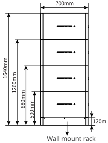
Battery group dimensions (wall-mount installation)
